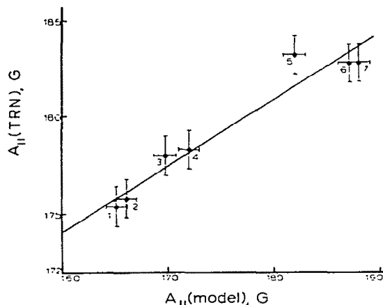
Fig. 10. Correlation of the parallel hyperfine splittings, A_{||} , between \text{VO}^{2+} -transferrin-anion complexes and simple model complexes employing the anion as a ligand. Data for the \text{VO}^{2+} -transferrin-anion complexes are for the B conformation. The linear regression line with a correlation coefficient of 0.978 is shown. 1. thioglycolate 2. thiosalicylate 3. phenyllactate 4. lactate 5. salicylate 6. oxalate 7. malonate. (R.F. Campbell and N.D. Chasteen, submitted for publication.)
